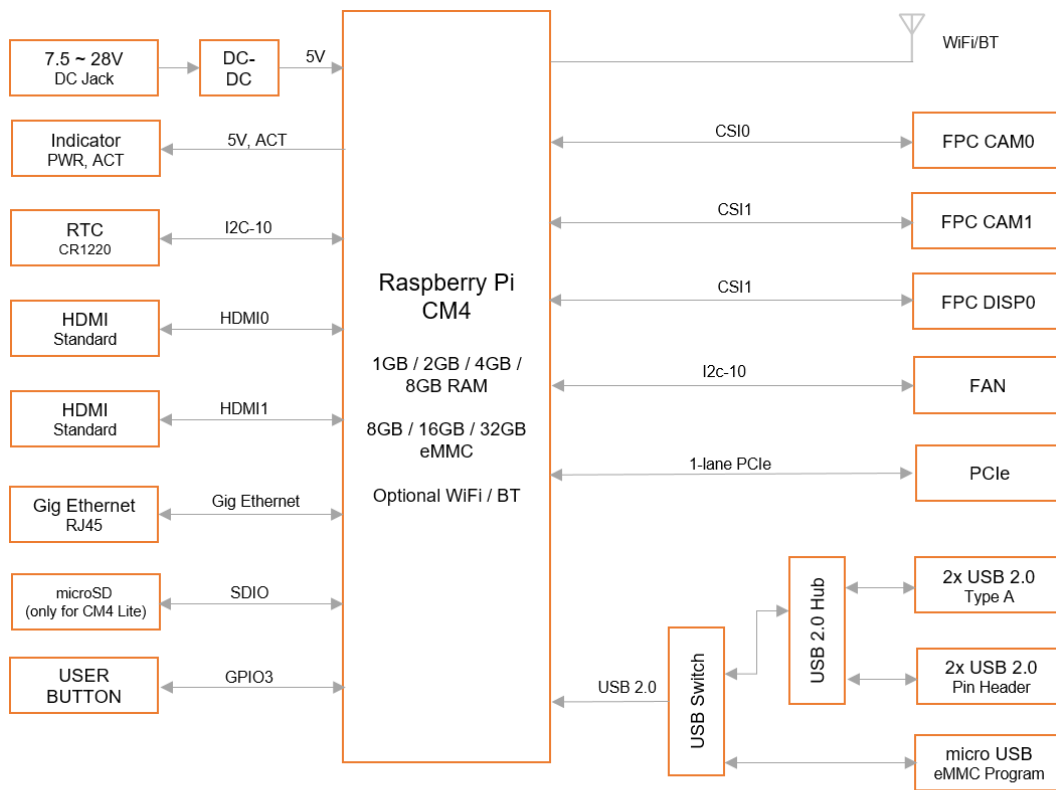
ED-CM4IO Computer
